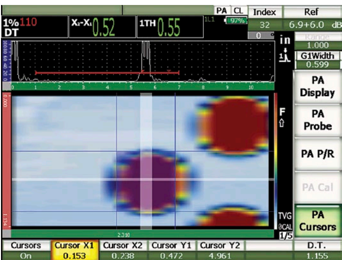
Zero-degree C-scan
